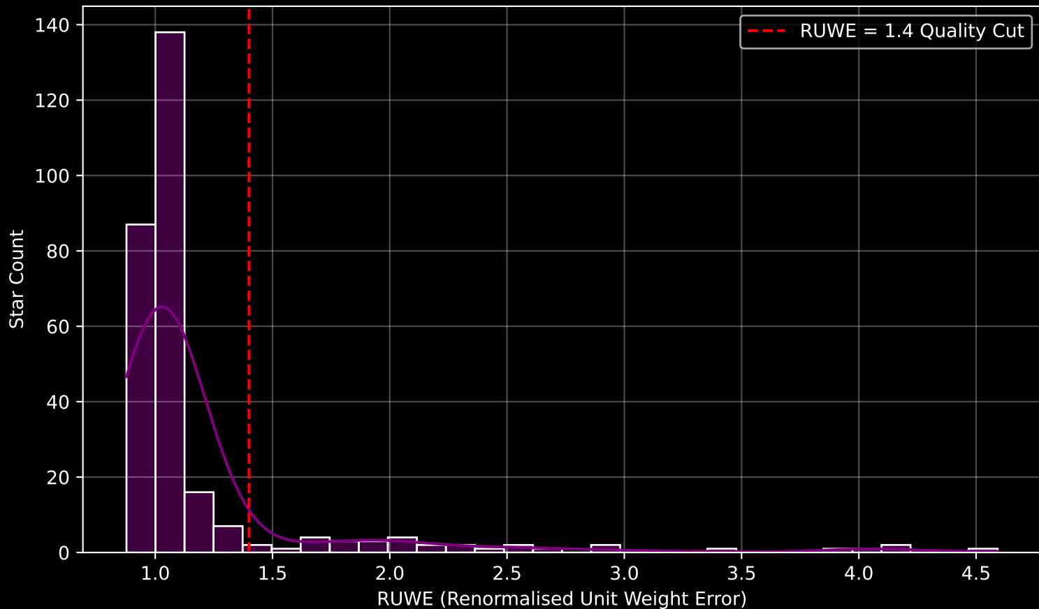
GALAH DR4 Field [887] RUWE Distribution (n= 281)
