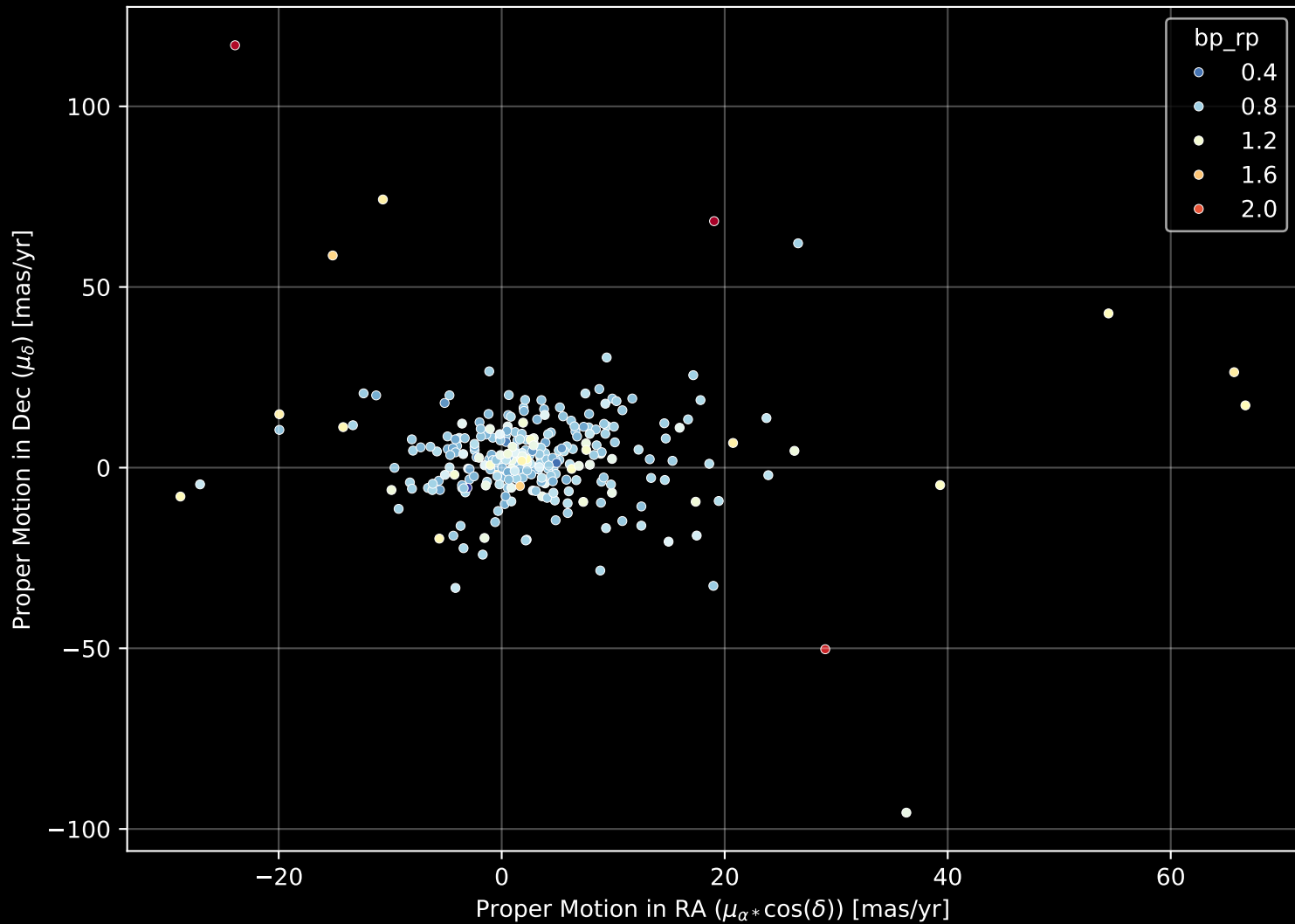
GALAH DR4 Field: [887] Proper Motion Diagram (n= 290)
