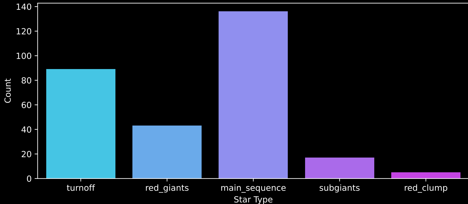
GALAH DR4 Field: [887] Count plot of Star Type
