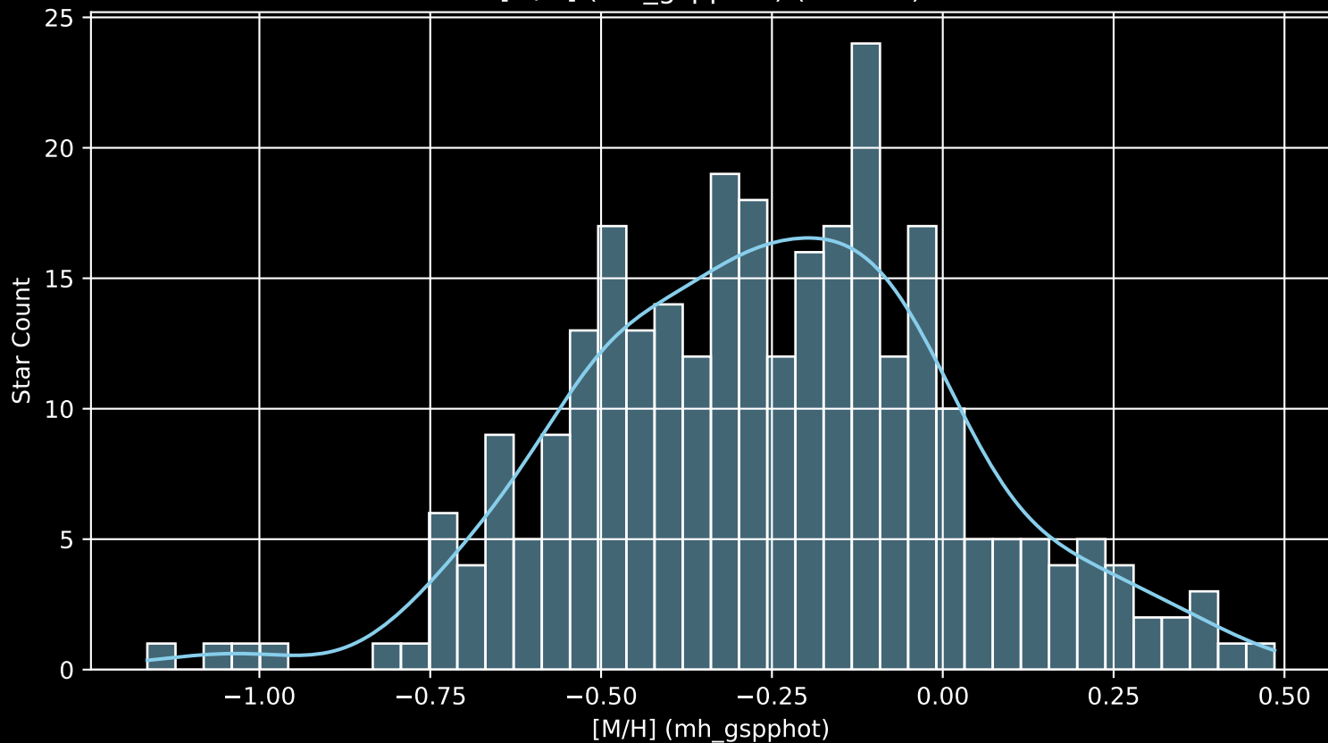
GALAH DR4 Field: [887] [M/H] (mh_gspphot) (n= 290)
